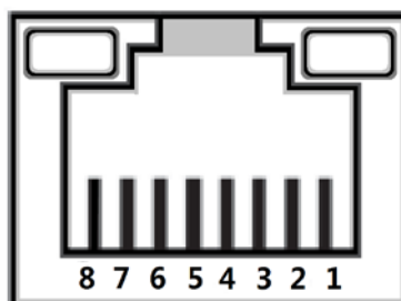
Figure 4-2 Ethernet port pin number
