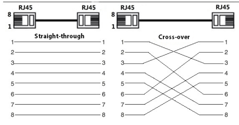
Figure 4-3 Connect cable
