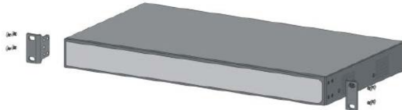
Figure 3-1 Install bracket
