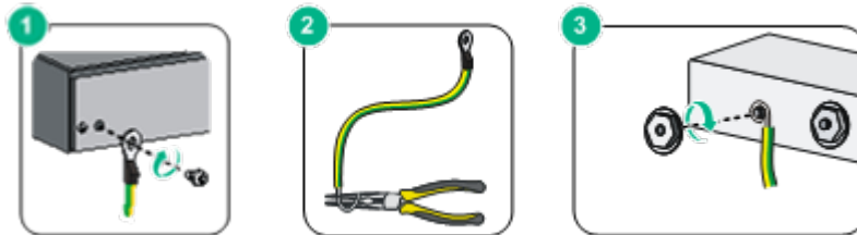
Figure 4-1 Connect GND
